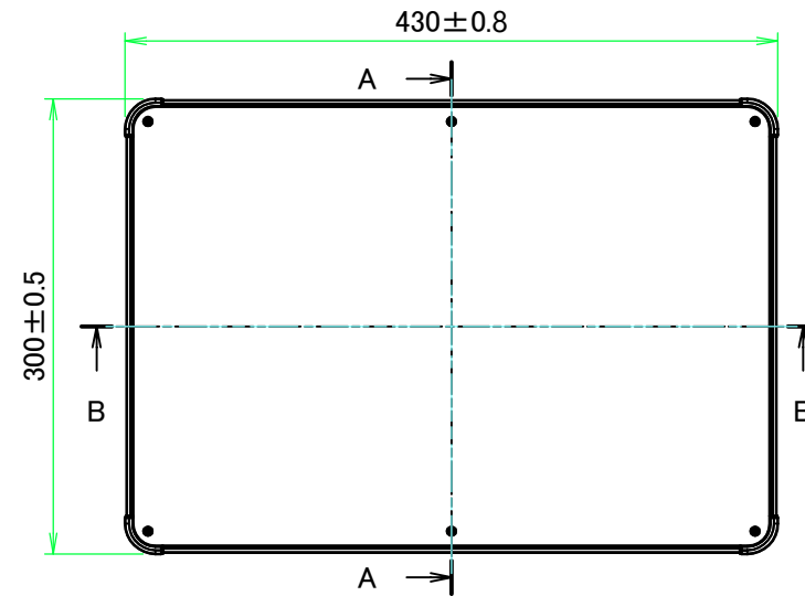
E view
